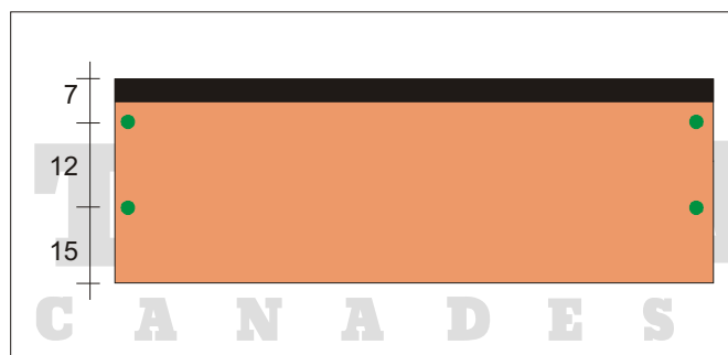
Picture Nr. 5 - How to nail the first row of shingles
