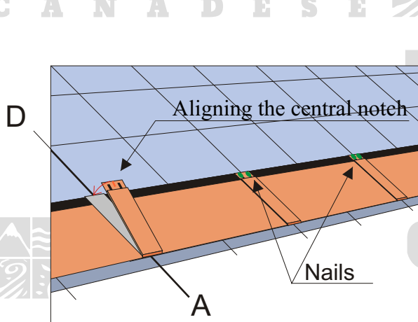
Picture Nr. 8 - Installation of Compact Clip
